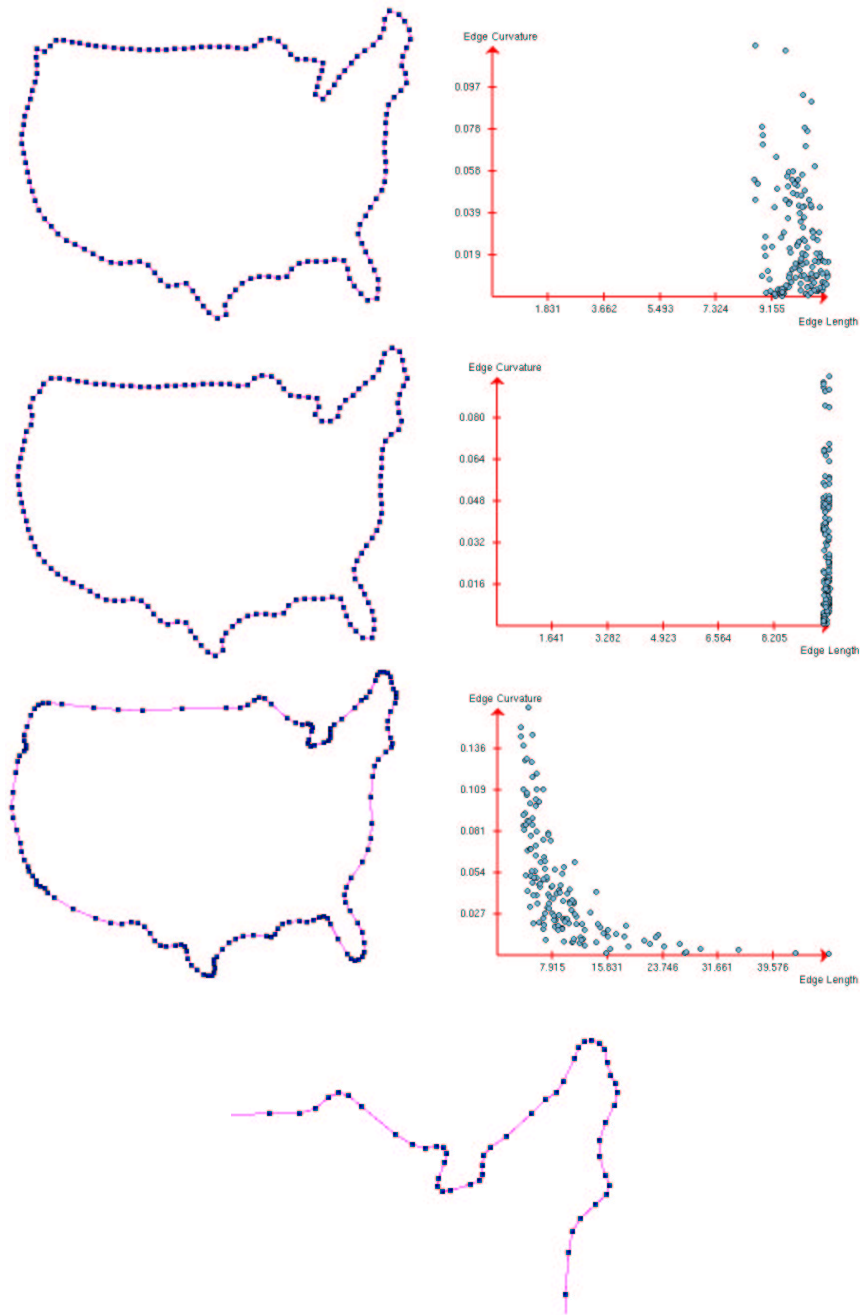
Figure 4: ( first row ) The initial contour with the edge curvature-length diagram; ( second row ) contour after applying the uniform vertex spacing tangential force. All edges have nearly the same length; ( third row ) contour after applying the curvature-based vertex spacing tangential force. The edge curvature is inversely proportional to edge length; ( fourth row ) enlarged view of the previous contour.
