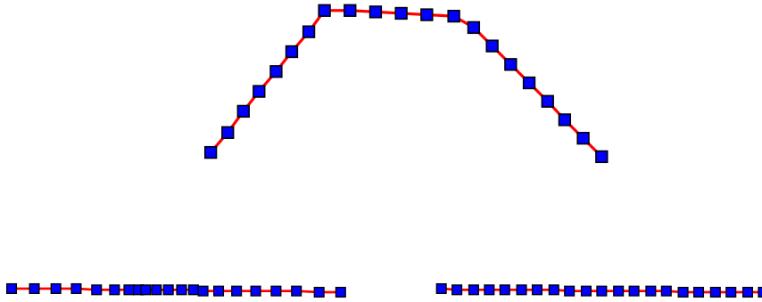
Figure 5: (top) Initial contour fixed at its two end vertices (bottom left) Equilibrium position after applying the Mean Curvature Motion : vertices are unevenly spaced; (bottom right) Equilibrium position after applying the Laplacian Smoothing : vertices are evenly spaced;
