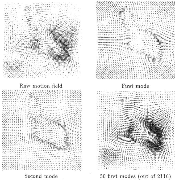
Figure 11. Modal approximation on 2D heart data. From up to bottom and left to right: the original motion field corresponding to the heart contraction, the two more representative modes and the field approximated by addition of the fifty more representative modes.
