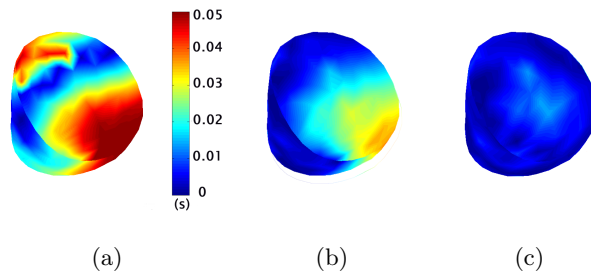
Fig. 7. Absolute depolarization time error between measures and simulations before (a) and after (b) the global automatic estimation and finally after the local estimation (c)
