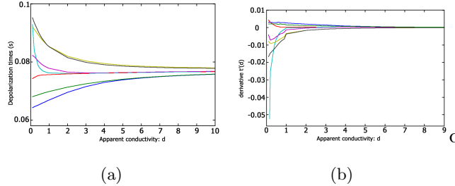
Fig. 12. (a) Depolarization time as a function of the apparent conductivity d_R at the seven vertices of a region R . (b) the derivative \partial t / \partial d of these curves
