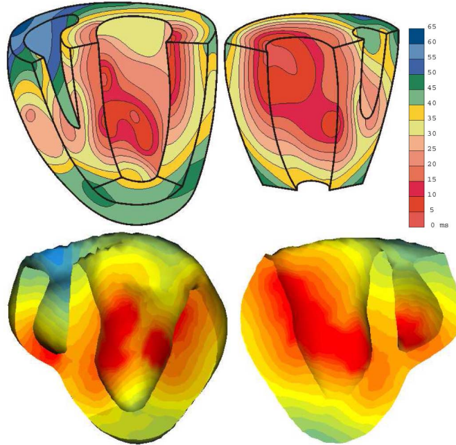
Fig. 9. Transmembrane potential isochrones (in ms) measured by Durrer et al. (top row) compared with the simulated ones (bottom row), on the UCSD geometry.
