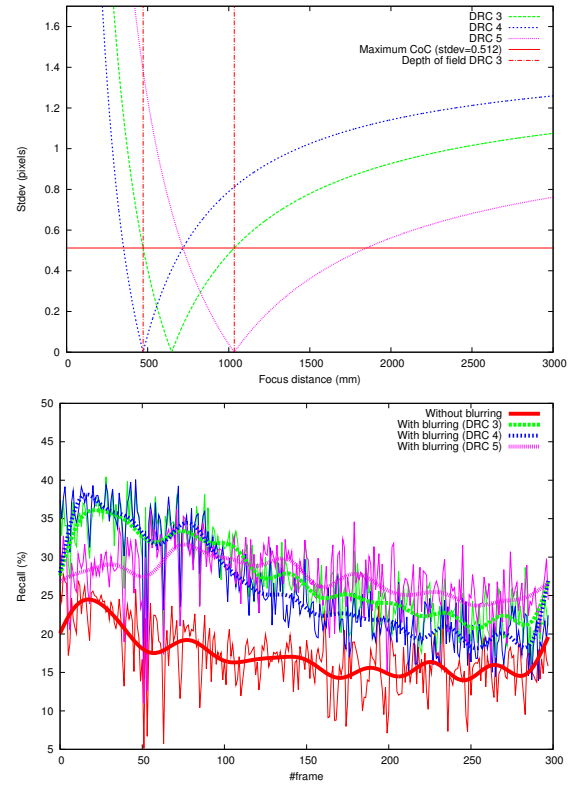
Figure 5: Sensitivity against DRC accuracy. Top to bottom : (a) DRCs obtained at the extremities of the depth of field (DRCs 4 and 5) and at focus distance (DRC 3) of the Poster sequence. (b) Recall values obtained over the Poster sequence using DRCs 3, 4 and 5 and without blurring.
