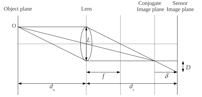
Figure 2: The ideal thin lens model.
