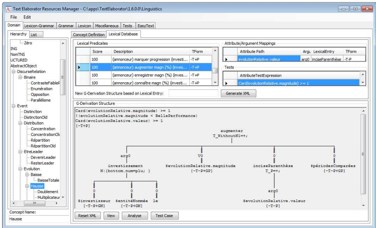
Figure 3: Scenshot of TextElaborator’s integrated development environment
