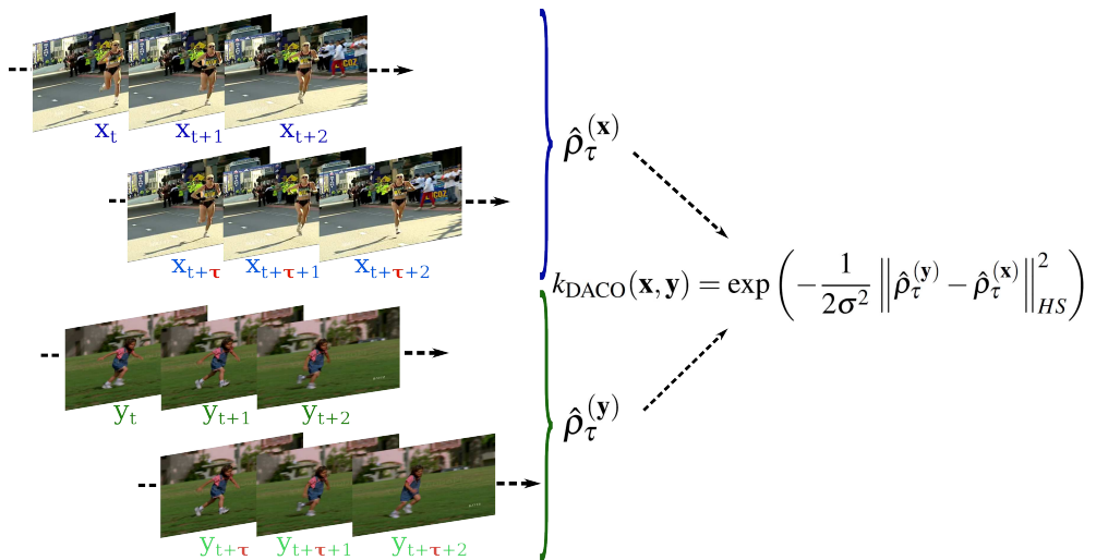
Figure 1: Computation of our DACO kernel. For two actions represented as time series of frames, \mathbf{x} = (x_1, \dots, x_{T'}) and \mathbf{y} = (y_1, \dots, y_{T'}) , the kernel compares their dynamics by using the difference between their auto-correlations \hat{\rho}_\tau^{(x)} and \hat{\rho}_\tau^{(y)} , with a lag of \tau frames.
