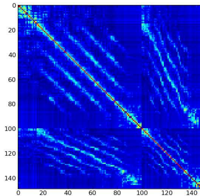
Figure 2: Example of a kernel matrix \mathbf{K} (c.f. equation 5) of kernel evaluations between the frames of two “walking” actions from the KTH dataset. “Warmer” colors represent higher similarity, the axes represent time (in frames) and the four blocks correspond to (from top-left to bottom-right) \mathbf{K}^{(x)} , \mathbf{K}^{(x,y)} , \mathbf{K}^{(y,x)} and \mathbf{K}^{(y)} . Note that actions are both periodic and display similar structures (visible in off-diagonal blocks).
