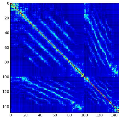
Figure 2: Example of a kernel matrix \mathbf{K} ( c.f. equation 5) of kernel evaluations between the frames of two “walking” actions from the KTH dataset. “Warmer” colors represent higher similarity, the axes represent time (in frames) and the four blocks correspond to (from top-left to bottom-right) \mathbf{K}^{(x)} , \mathbf{K}^{(x,y)} , \mathbf{K}^{(y,x)} and \mathbf{K}^{(y)} . Note that actions are both periodic and display similar structures (visible in off-diagonal blocks).
