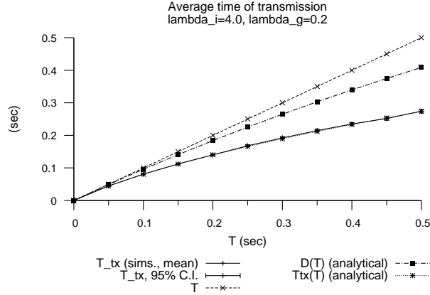
Figure 7: Average time to transmission for \lambda_{in} = 4 \frac{pkt}{s} , \lambda_g = 0.2 \frac{pkt}{s} , for different values of t (simulations and analytical results).
