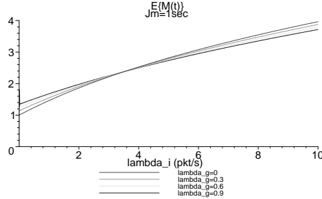
Figure 5: Mean of M(t) (w.r.t. t ) depending on \lambda_{in} , for different values of \lambda_g , J_m = 1sec .
