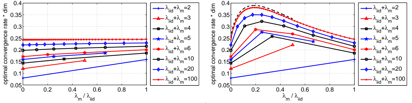
Figure 3: Optimal asymptotic convergence rates CR^{opt, \infty}(\lambda_{iid}, \lambda_m) , Equation (24), for the (\mu/\mu_w, \lambda_{iid} + \lambda_m) -ES versus the ratio \lambda_m/\lambda_{iid} of mirrored and independent offspring for various \lambda = \lambda_{iid} + \lambda_m . Left: (\mu/\mu_w, \lambda_{iid} + \lambda_m^{rand}) -ES with random mirroring. Right: (\mu/\mu_w, \lambda_{iid} + \lambda_m^{sel}) -ES with selective mirroring, mirroring the worst \lambda_m from \lambda_{iid} independent offspring. In addition, the righthand plot shows the theoretical result for \lambda_{iid} \rightarrow \infty of Equation (25) as a dashed line.
