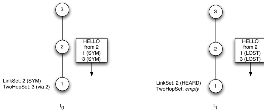
Figure 6: Graceful shutdown
