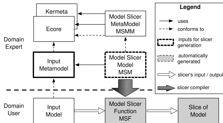
Fig. 2. Overview for Modeling Model Slicers with Kompre
