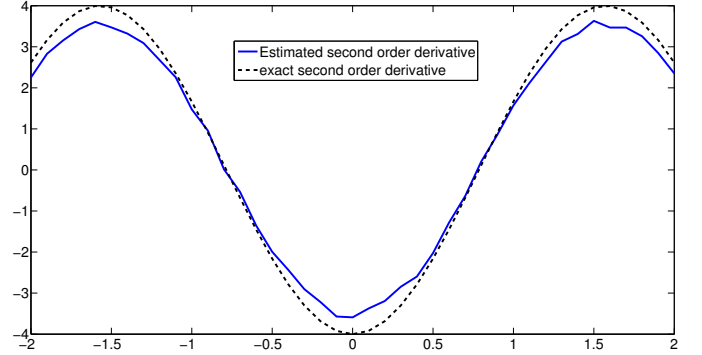
Fig. 4. Exact (dashed line) and estimated (solid line) values of \frac{\partial^2 \mathcal{T}}{\partial x^2} .
