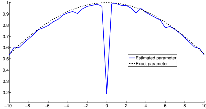
Fig. 6. Exact (dashed line) and estimated (solid line) thermal conductivity.
