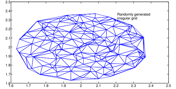
Fig. 3. A randomly generated grid used for the estimation of \mathcal{T}_x with (x - 2)^2 + (y - 2)^2 < 0.15 .
