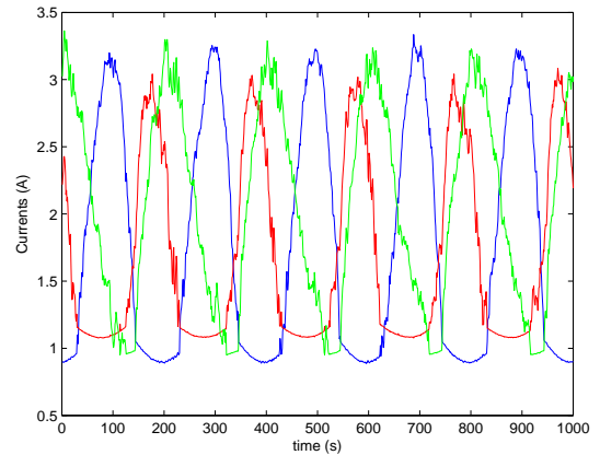
Fig. 5. Control Currents
