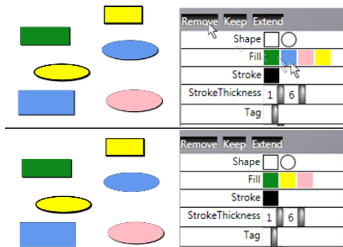
Figure 10: The user drags the Remove instrument and drops it on the blue fill shared value. All blue objects are removed from the selection.
