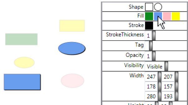
Figure 7: The user's cursor is over the blue shared value of the fill property (fill: blue). Because they don't have this shared value, the green rectangle, the pink circle and the two yellow shapes are dimmed
