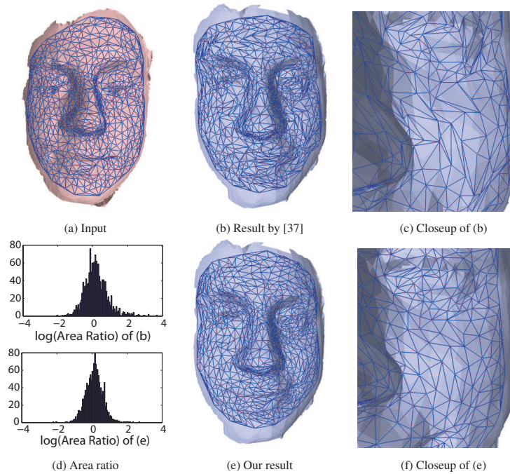
Figure 6: Shape registration result. (a) shows the input mesh with triangulated discrete samples obtained by the method described in [37]. The matching result and its closeup is shown in (b) and (c).
