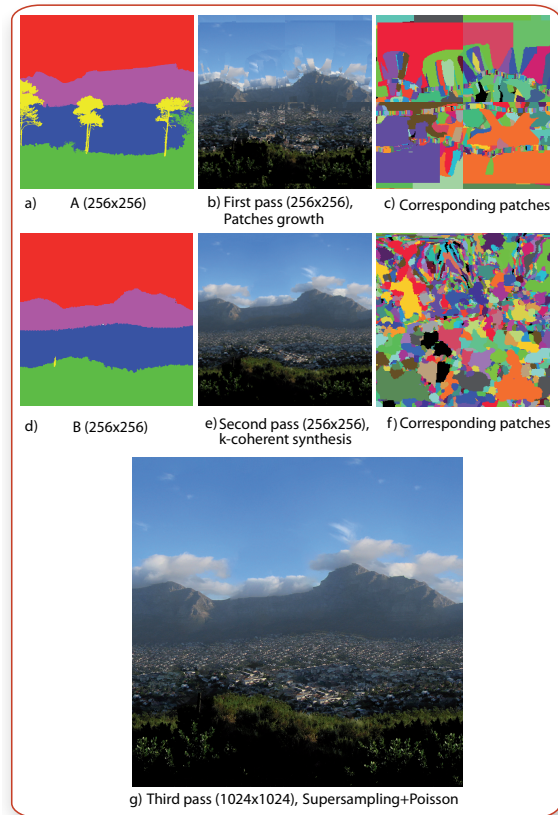
Figure 6: Our parallel three-step guided synthesis pipeline. Image A represents the labels in the input photo, while B are the synthesized labels from the proxy guide. The input photograph can be seen in Fig.7 of the additional material.
