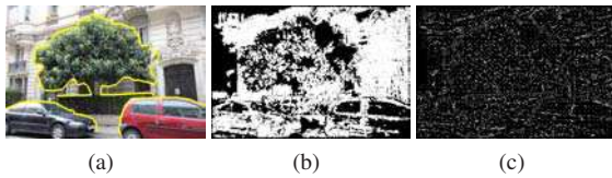
Figure 2: (a) Silhouettes marked at sharp depth differences; (b) Original reconstructed point cloud with 118,049 points; (c) Sparse uniform point cloud with 6324 points selected by our approach. Note the regions with no original 3D points are also filled with new points (see Sec. 4.2).
