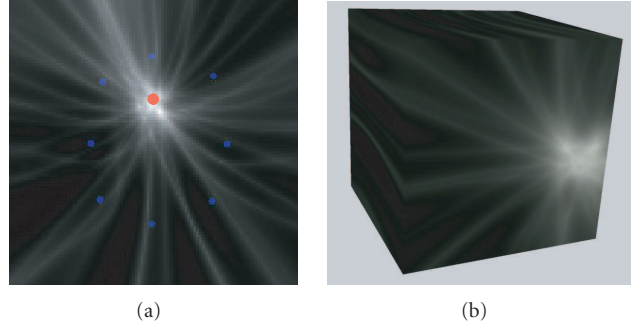
FIGURE 6: (a) A 2D probability histogram for source location obtained by sampling a weighted sum of hyperboloids corresponding to the time-difference of arrival to all microphone pairs (shown in blue). We pick the maximum value (in red) in the histogram as the location of the frequency band at each frame. (b) A cut through a 3D histogram of the same situation obtained by sampling hyperboloid surfaces on a 3D grid.
