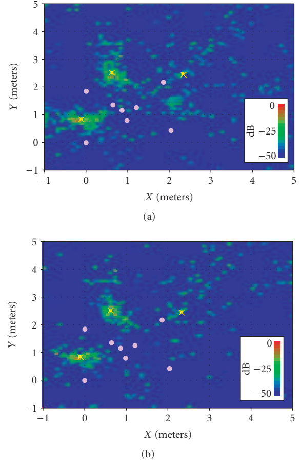
FIGURE 8: Energy localization map for a 28 s.-long audio sequence featuring 3 speakers inside a room (indicated by the three yellow crosses). Light-purple dots show the location of the 8 microphones. The top map is computed using AMDF-based TDOA estimation while the bottom map is computed using GCC-PHAT. Both maps were computed using 8 subbands and corresponding energy is integrated over the entire duration of the sequence.
