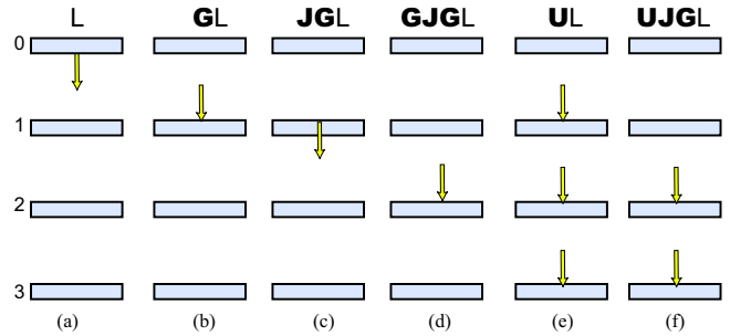
Figure 4: Radiance after unoccluded transport \mathbf{U} is the sum of radiance after a series of occluded transport \mathbf{G} and “go-through” \mathbf{J} .
