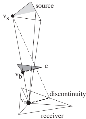
Fig. 18. Degeneracy due to discontinuity meshing. The receiver is split along discontinuity v_r e , causing a degenerate v_s v_b v_r extremal stabbing line.
