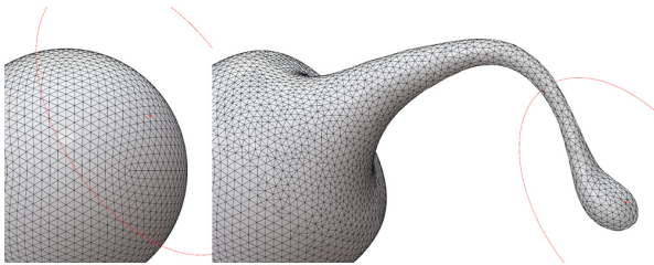
FIGURE 11: Volume-preserving sweep deformation applied to a quasi-uniform spherical mesh.
