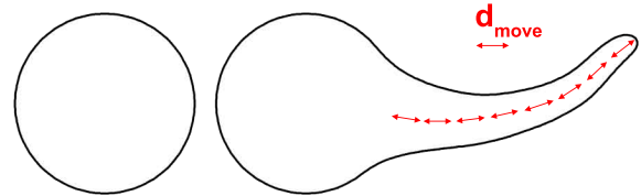
FIGURE 9: Sweep deform. The original large deformation is divided into elementary steps (red segments) to limit the maximum displacement to d_{move} .
