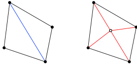
FIGURE 1: Edge split. As the blue edge splits into two equal segments, the four created edges in red are smaller than the largest initial edge.
