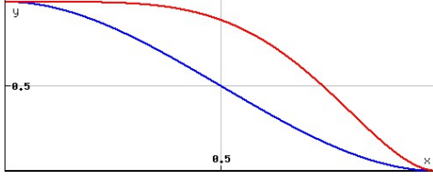
FIGURE 13: Blend function for n = 3 (blue) and n = 6 (red).
