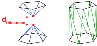
FIGURE 6: Vertex join. When two non adjacent vertices get within d_{thickness} of each other, the surface changes topology by deleting them and reconnecting the remaining 1 - rings .
