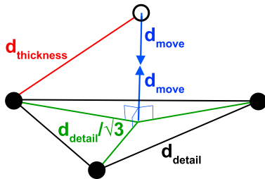
FIGURE 4: d_{move} is chosen so that a vertex approaching a non incident face that is moving in the opposite direction, is not allowed to pass through.
