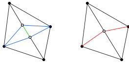
FIGURE 2: Edge collapse. This operation is performed if the size of the green edge is smaller than d .
