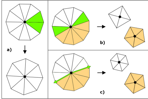
FIGURE 16: Cleanup on the triangle fan around the affected vertex (in black). Degenerate components are schematically shown in green and should be considered collapsed over each other. For simplicity they are represented as separate components in the neighborhood. The procedure is applied as follows : a) Degenerate consecutive facets in the fan are deleted. b) Degenerate non-consecutive facets are deleted and the central vertex is split. c) Degenerate edges split the neighborhood in two regions.
