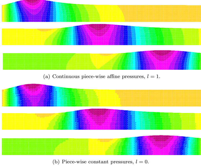
Figure 1: Snapshots of the pressure at t = 0.005, 0.01, 0.015 (from top to bottom). Algorithm 4 with \mathbf{d}_h^* = \mathbf{d}_h^{n-1} , \tau = 10^{-4} and h = 0.05 . Fluid domain in deformed configuration (amplified).
