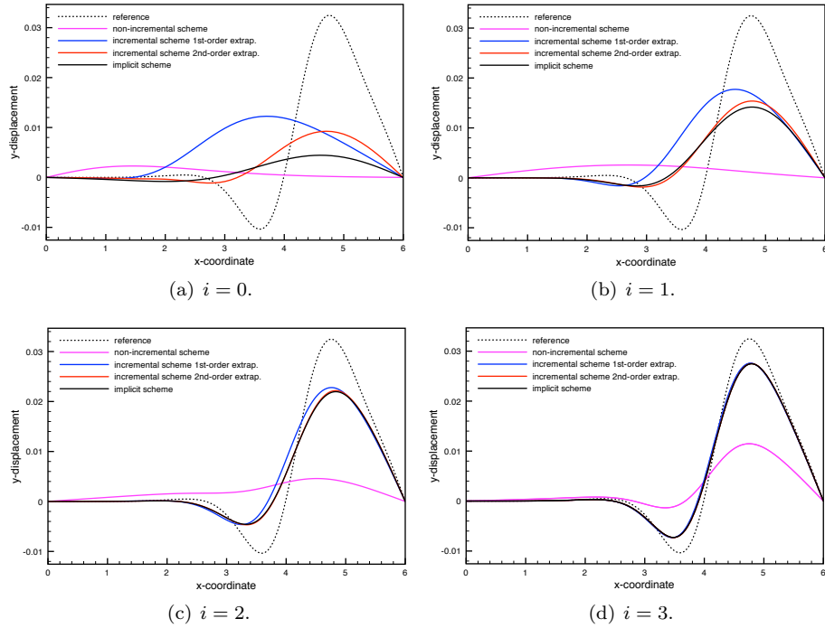
Figure 4: Comparison of the displacements at t = 0.015 , obtained with k = l = 1 and different levels of (\tau, h) -refinement, given by (80) with i = 0, \dots, 3 .
