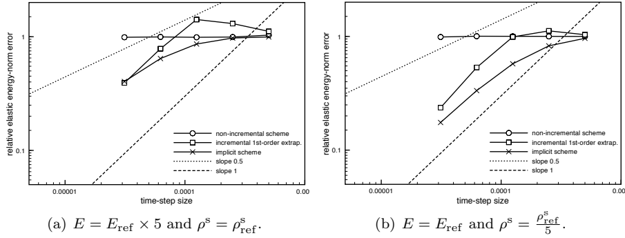
Figure 6: Displacement energy-error convergence history in time for a higher \omega^e .
