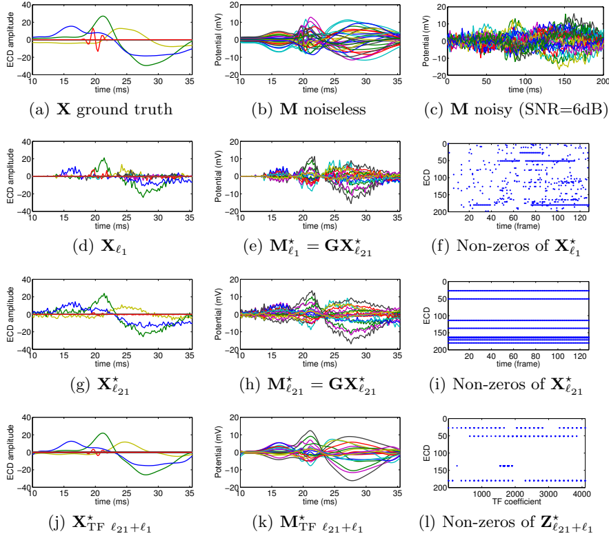
Fig. 3. Simulations results with SNR = 6 dB. (a) simulated source activations. (b) Noiseless simulated measurements. (c) Simulated measurements corrupted by noise. (d-e-f) Estimation with \ell_1 prior. (g-h-i) Estimation with \ell_{21} prior [20]. (j-k-l) Estimation with composite TF prior. (f-i-l) show the sparsity patterns obtained by the 3 different priors as explained in Fig. 1. Result (j) shows how the composite TF prior improves over (d) and (g). (l) presents also a higher level of sparsity compared to (f) and (i).
