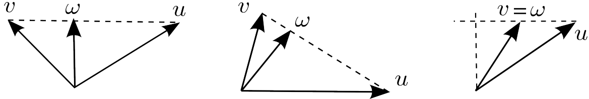
Figure 1: Various possible configurations of the two gradient-vectors u and v and the minimal-norm element \omega .
