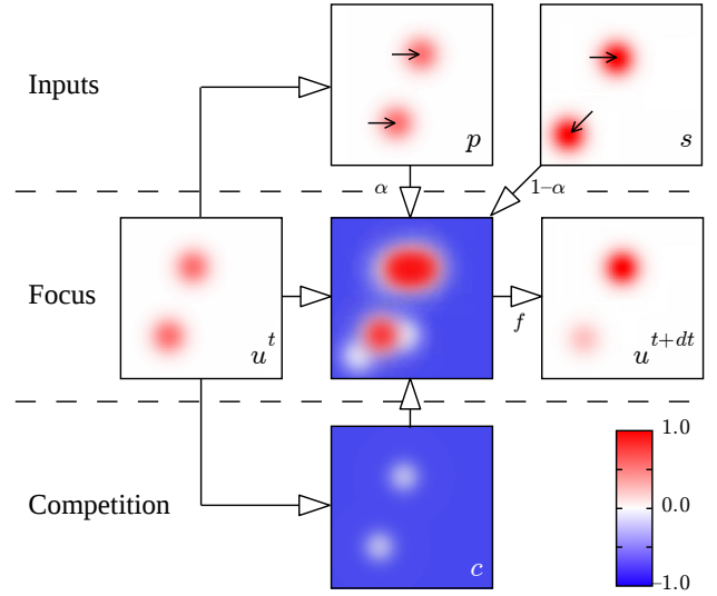
Fig. 1. Graphical illustration of the predictive CNFT dynamics. Although 2 bubbles are competing for the focus on the field u^t , a single stimuli from the stimulation s confirms the rightward translation anticipated by the predictor p (predicted and actual movements are indicated by arrows). Combining the different fields (terms in Eq. 1) and applying the non linear function f gives the new focus activity u^{t+dt} , the inhibitory field induced by the competition eliminating most non coherent activities. Convergence thus occurs on the stimulus that matches the prediction.
