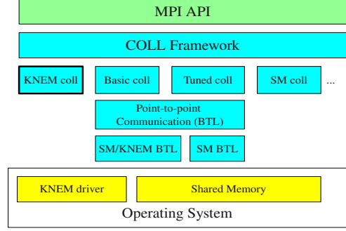
Figure 2. Open MPI collective communication framework
