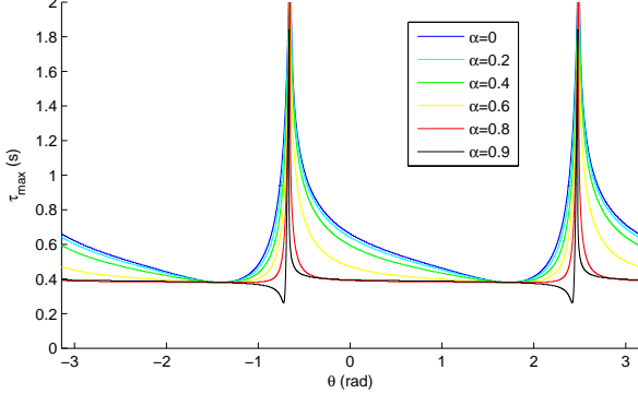
Fig. 2. Example 1: State-angle dependent sampling function \tau for different decay rates \alpha .
