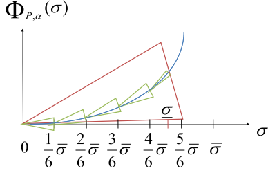
Fig. 4. Building polytope subdivisions (here with l = 6 )
