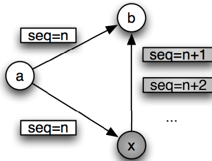
Figure 2: Pre-play attack: X is a malicious router, which generates invalid packets with valid sequence numbers.
