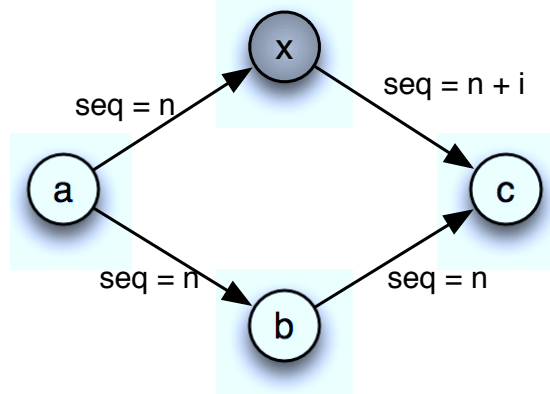
Figure 5: Sequence number attack. X is the malicious router and modifies the sequence number to disturb duplicate packet detection
