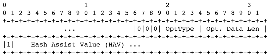
Figure 6: The Hash Assist Value header option in H-DPD mode
