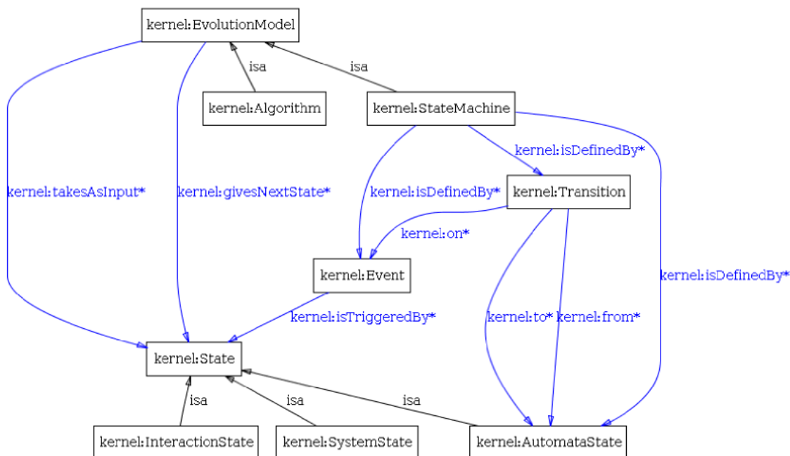
Figure 6: EvolutionModel.class
