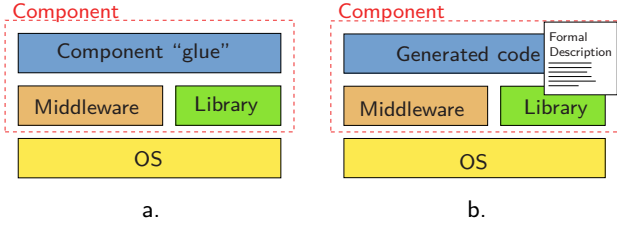
Fig. 1. a. A component architecture realizing a clear separation of concerns between a middleware and a library: glue code grants the decoupling. b. The G en M3 tool generates the glue code from a component formal description and a skeleton (not shown on the figure) suited to the middleware.
