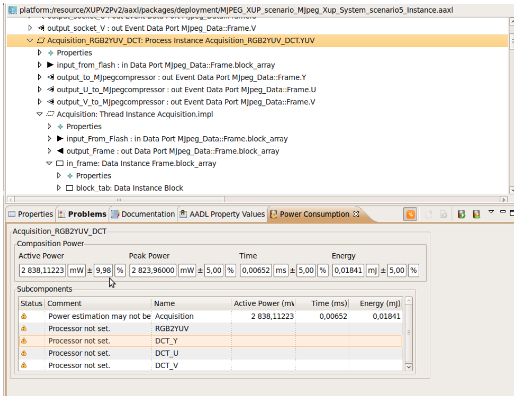
Figure 26 : Power consumption results view : display of uncertainty
