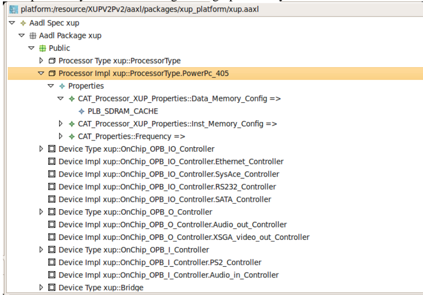
Figure 20 : CAT AADL object tree editor window
