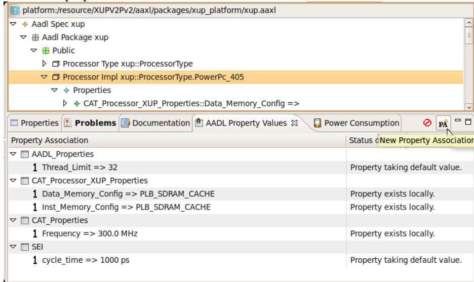
Figure 23 : AADL Property Values View
