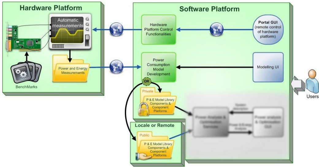
Figure 2 : The software platform: the PCMD functionalities
