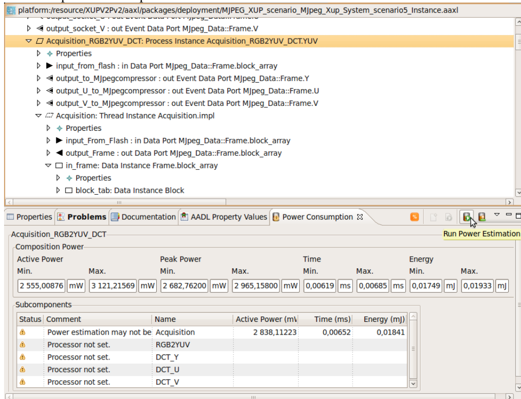
Figure 24 : Example of CAT Power consumption view
