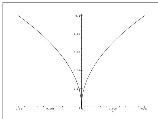
Figure 1: Singular signal with exponent 0.5
