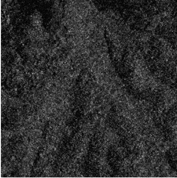
Figure 10: Multifractal image denoising, with shift parameter 0.3
