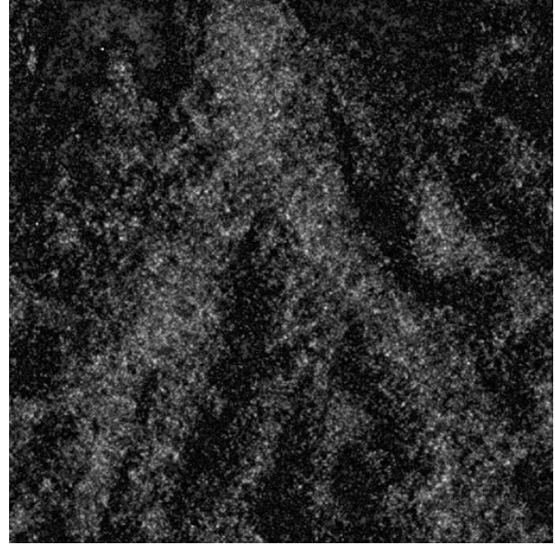
Figure 11: Multifractal image denoising, with shift parameter 0.5
