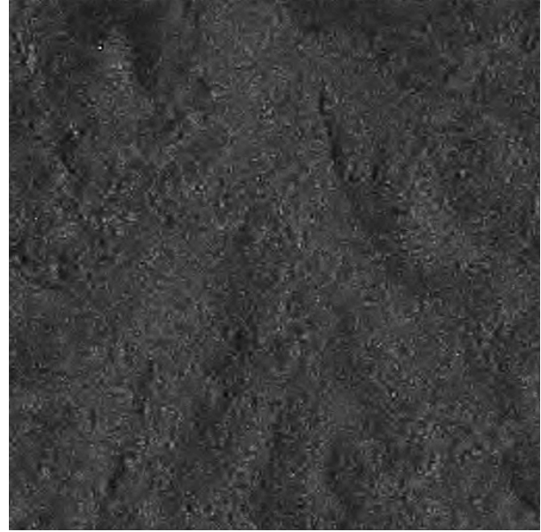
Figure 13: Denoising by wavelet coefficient thresholding
