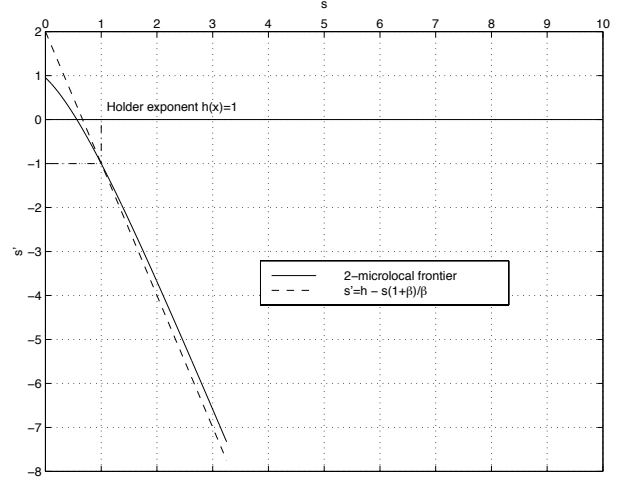
Figure 8: Relation between 2-microlocal domain and chirps exponents
