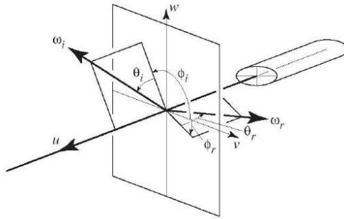
Figure 1.9: Light scattering notations [WBK + 07].
