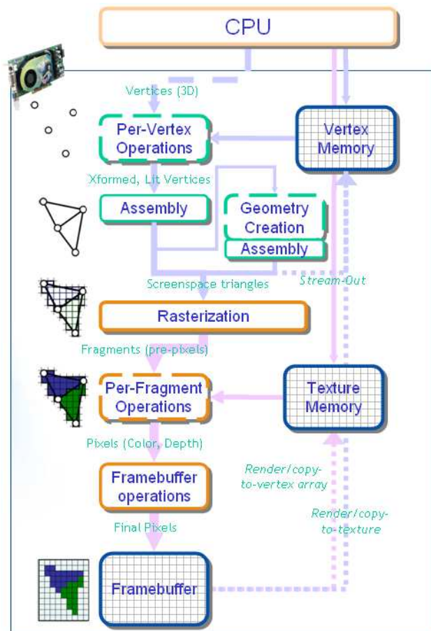
Figure 2.7: Graphics pipeline
