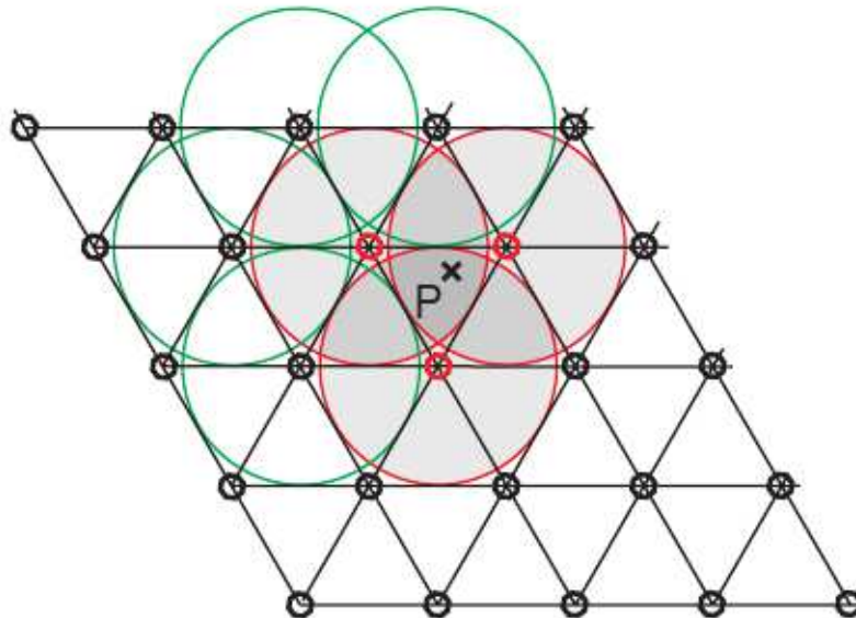
Figure 3.2: Fewer contribution of wavelets make the simplex grid more efficient (Gustavson, 2005)
