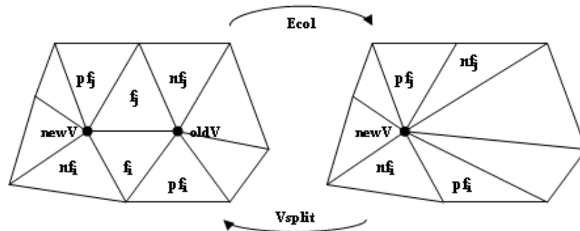
Figure 1 : Half Edge Collapse.
