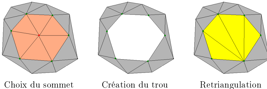
Figure 2 : Vertex Removal
