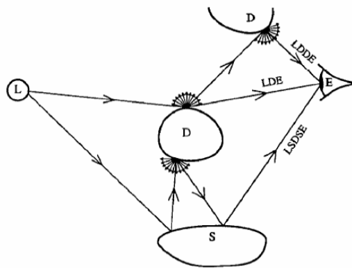
Figure 1 From Heckbert [1]. (L)ight. (S)pecular. (D)iffuse. (E)ye. See text.
