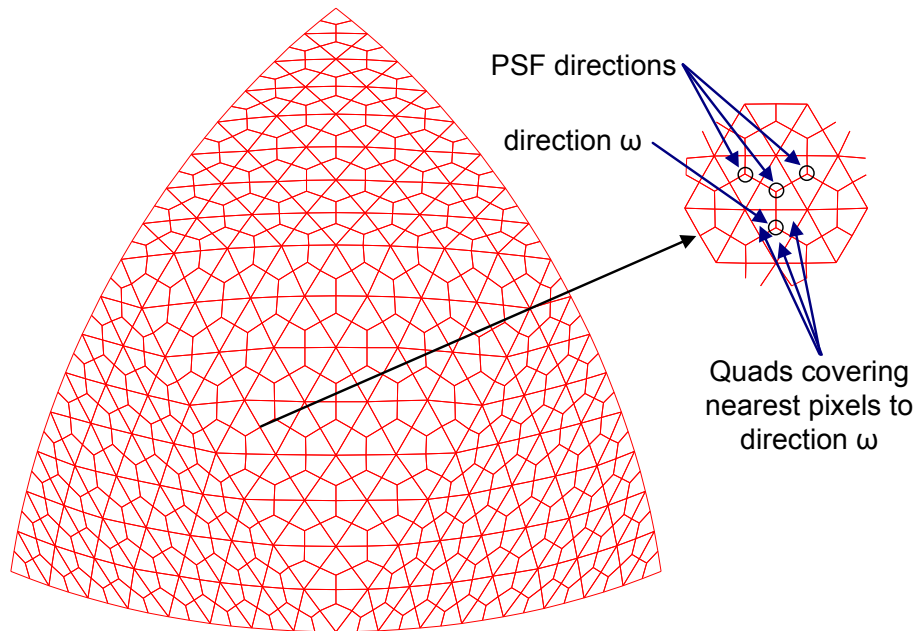
Figure 15 A Quadrant of the hemisphere used to lookup PSF directions (viewed from within). Note unequal solid angles.
