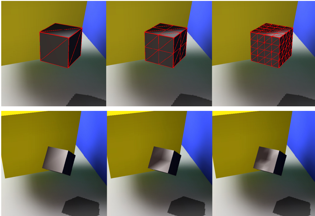
Figure 32 Upper row: triangle subdivision at levels 0,1,2. Lower row: the effects on shading
