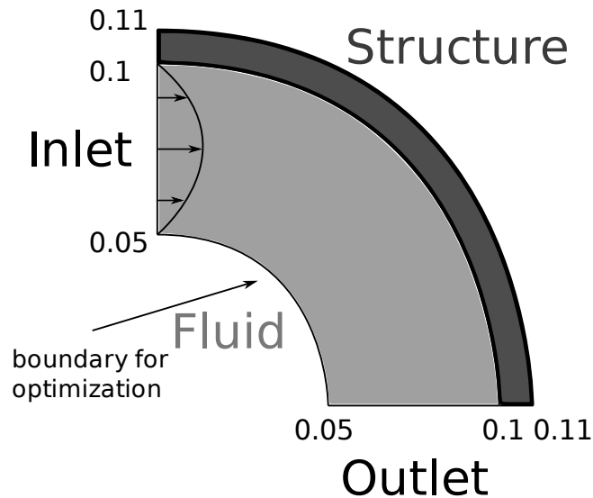
Figure 2: Initial geometry of FSI problem with fluid (light grey) and structural domain (dark grey)
