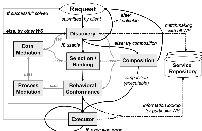
Fig. 1. Automated Web Service Usage with SWS
