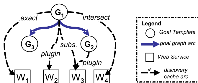
Fig. 4. Example of a SDC Graph
