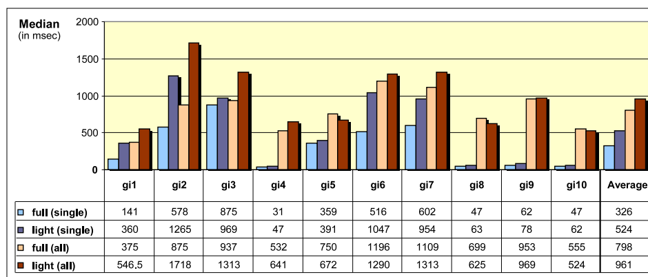
Fig. 11. Performance Comparison SDC vs. SDC light
