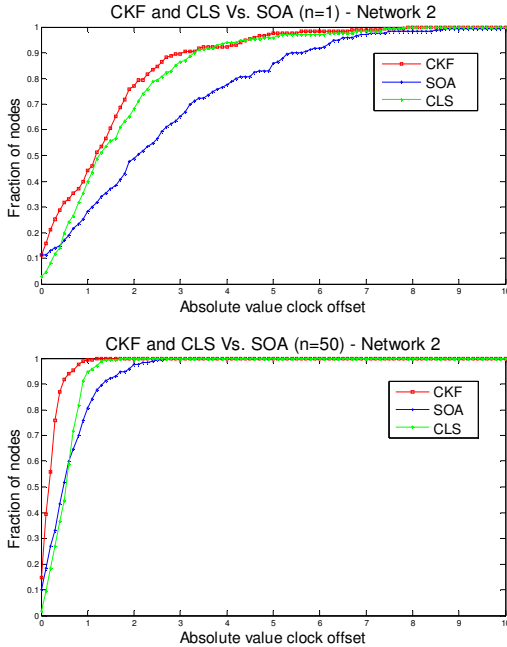
Figure 2. Comparison between CKF, SOA and CLS (with R \sim U[0.01,12] and P_0 \neq I ) in Network 2 for n = 1, 50 .
