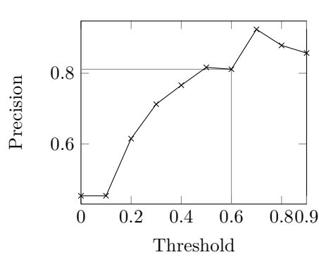
Figure 1: Precision of class alignment YAGO \subseteq DBPEDIA as a function of the probability threshold.
