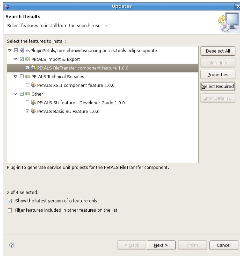
Figure 29: PEtALS installation
