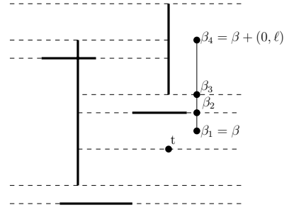
Figure 2: \mathcal{H} (bold), its extension T(\mathcal{H}, t) (dashed), and exit points E_t(\beta) of a highway
