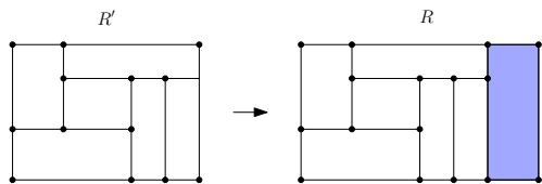
Figure 1: Extending a rectangular partition of odd order to a rectangular partition of even order.
