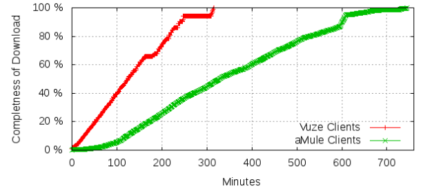
Fig. 7: Download Times with 1 Source.
