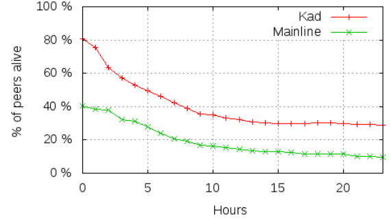
Fig. 3: Measured aliveness of nodes.
