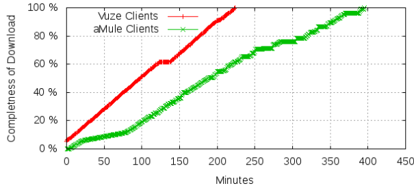
Fig. 9: Download Times with 10 Sources.
