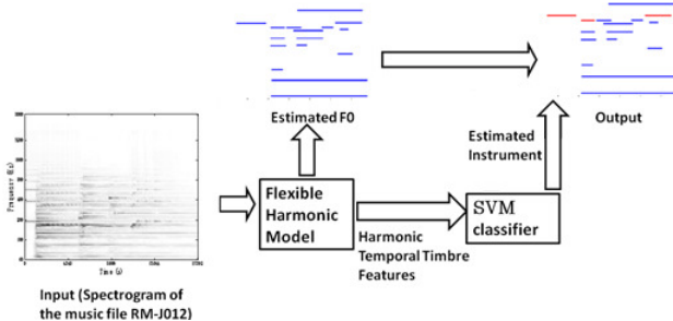
Figure 1. Flow chart of the proposed system.
