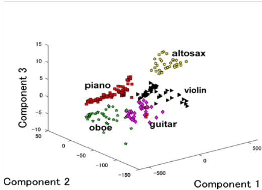
Figure 7. First three principal components of the proposed feature set with attack features.
