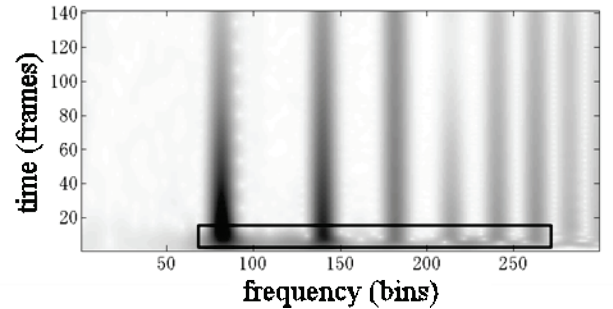
Figure 2. Spectrogram of a piano note signal. The rectangle marks the attack part of the note.
