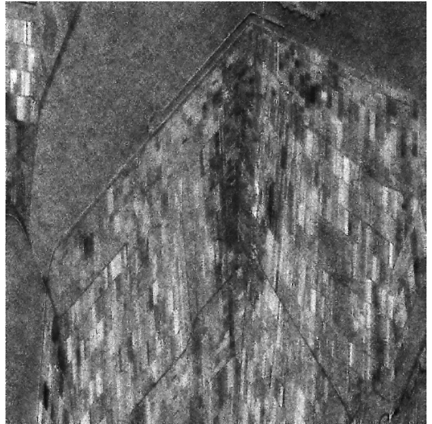
Figure 10: Denoising by multifractal spectrum distortion
