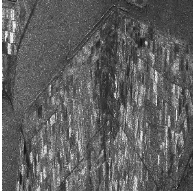
Figure 9: Denoising by wavelet shrinkage
