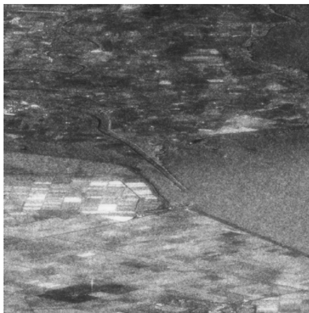
Figure 5: Denoising by multifractal spectrum shifting
